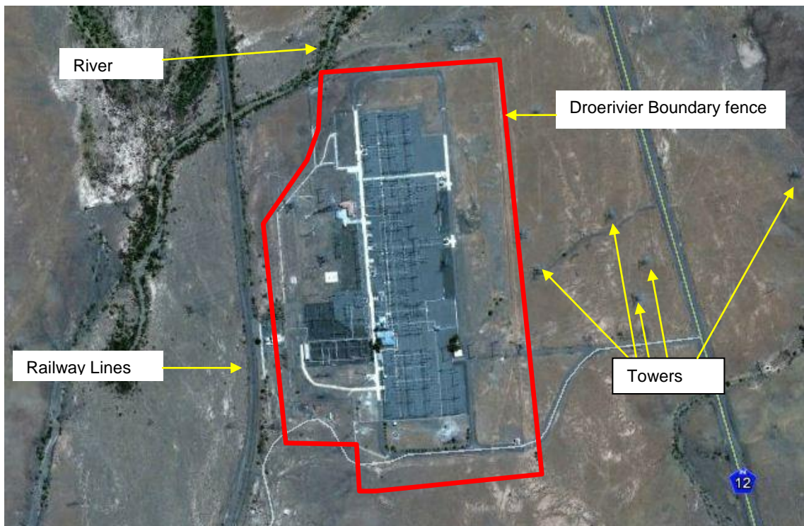
Figure 17. Droërvier Substation
